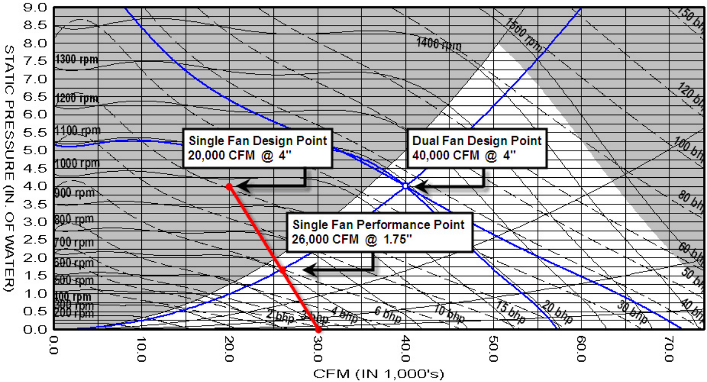
Figure 6: Dual Fan Redundancy – 65% If One Fan Fails
