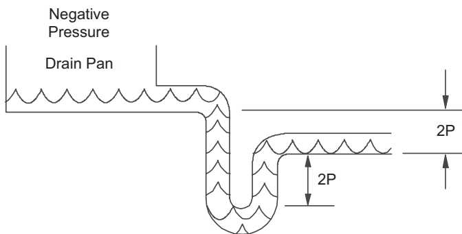
Figure 17: Drain Pan Traps
