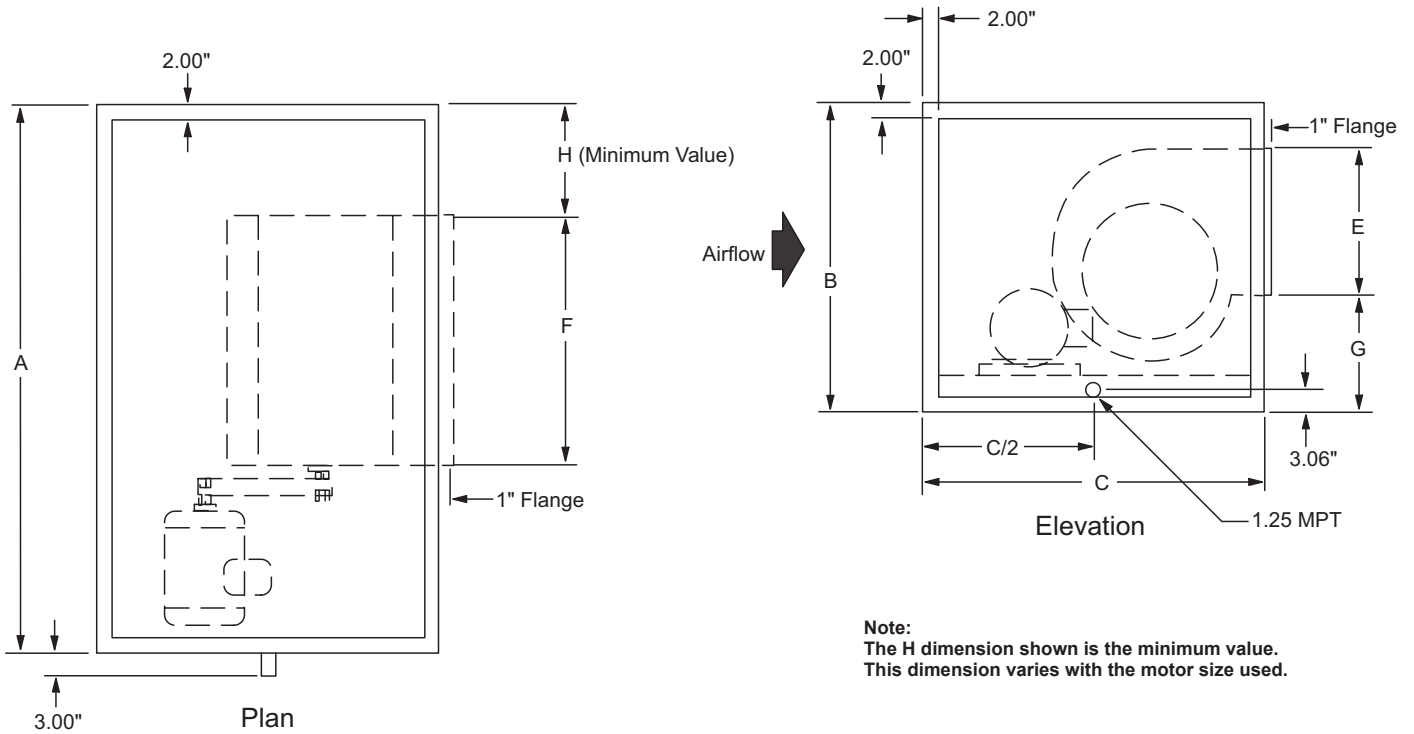
Figure 24: Dimensional Data—Top Horizontal Housed Fan Discharge
