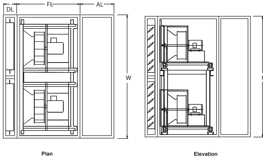
Figure 27: Dimensional Data—Fan Array Four Fan Model
