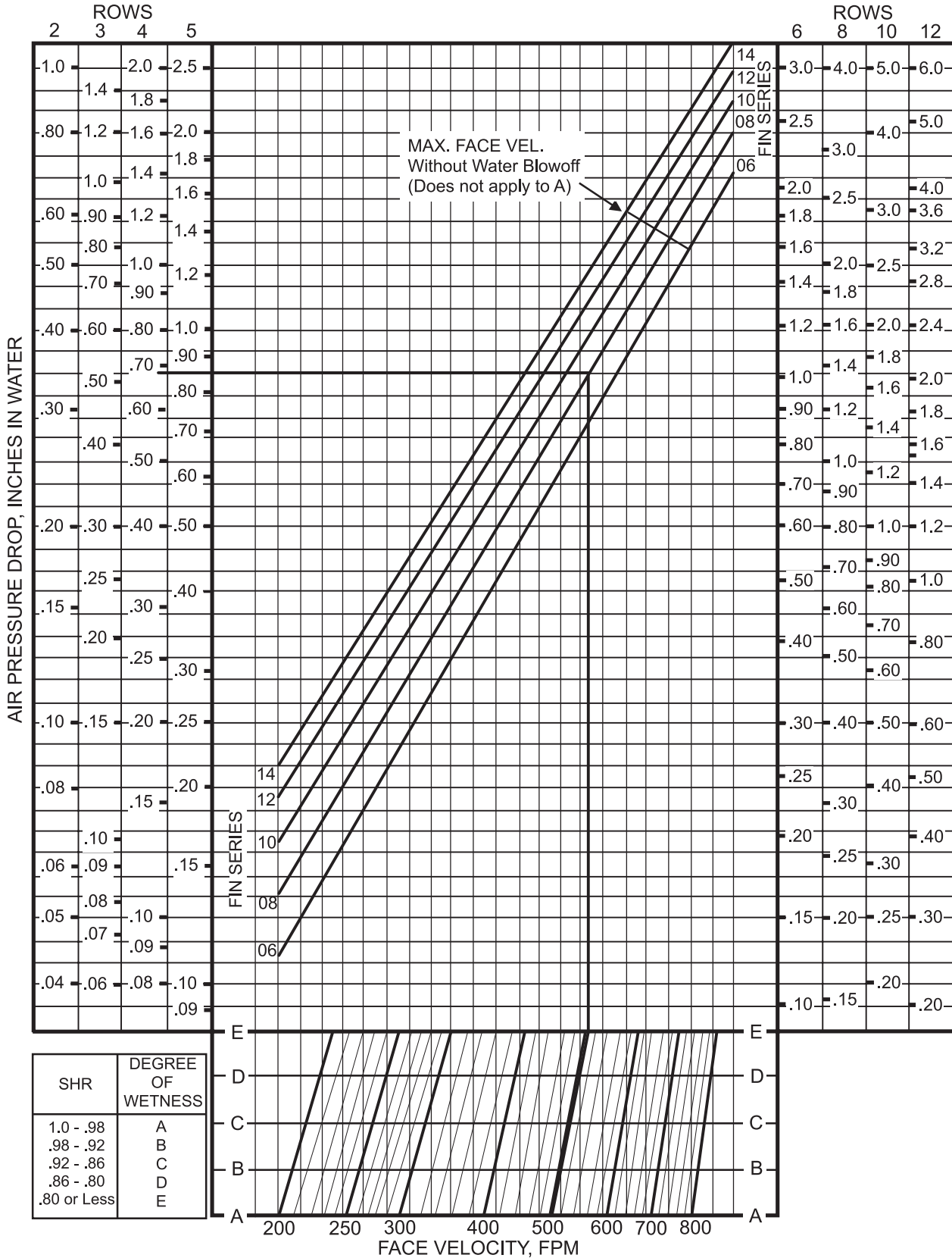
Figure 19: Coil Air Pressure Drop—HI-F5 Fin Type (2 Through 12 Rows)
