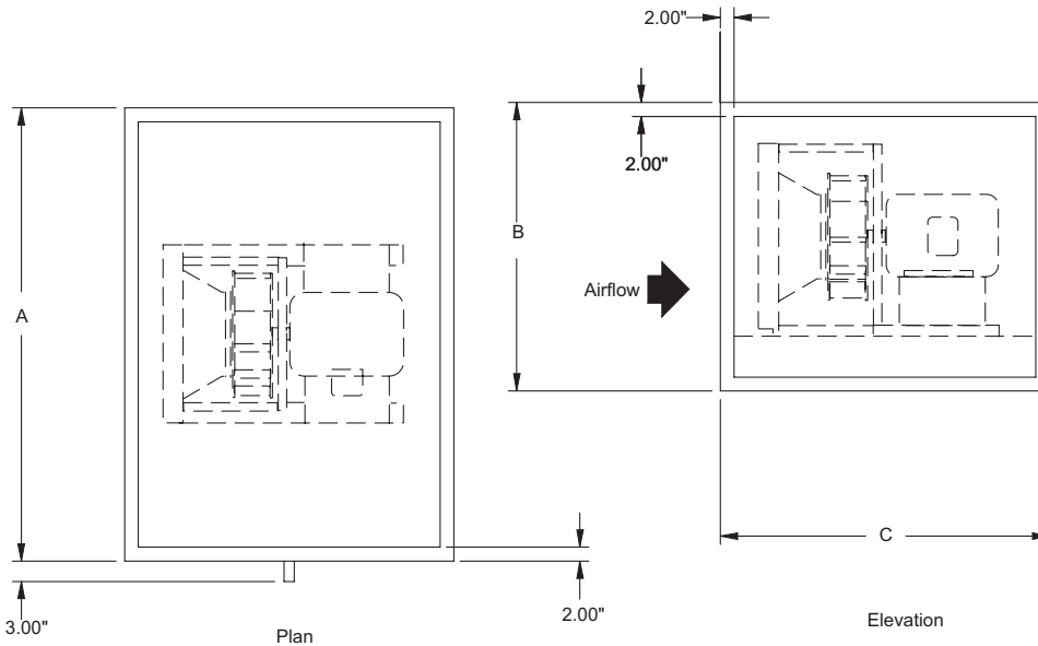
Figure 29: Dimensional Data—Direct-Drive Plenum Fan Discharge
