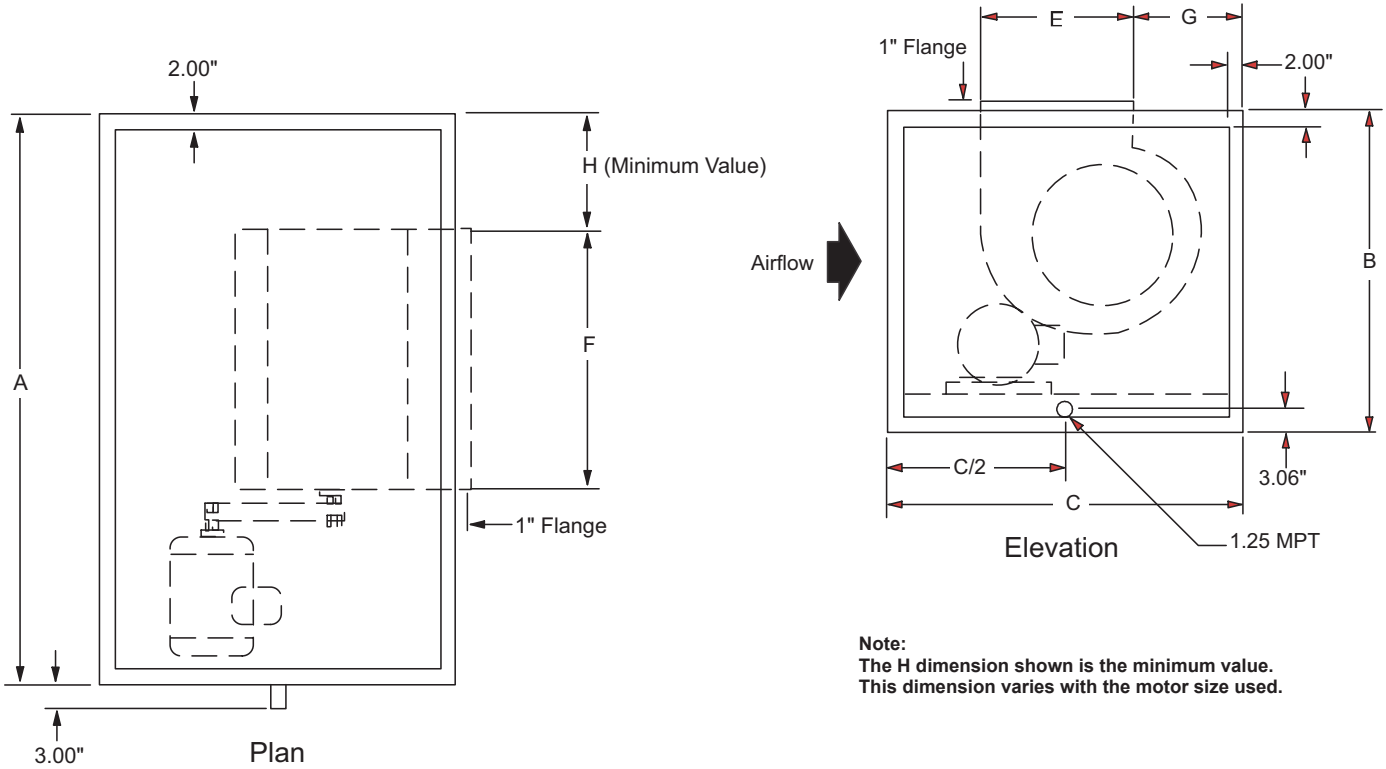
Figure 26: Dimensional Data—Upblast Housed Fan Discharge
