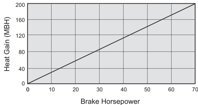
Figure 18: Fan and Motor Heat Gain
