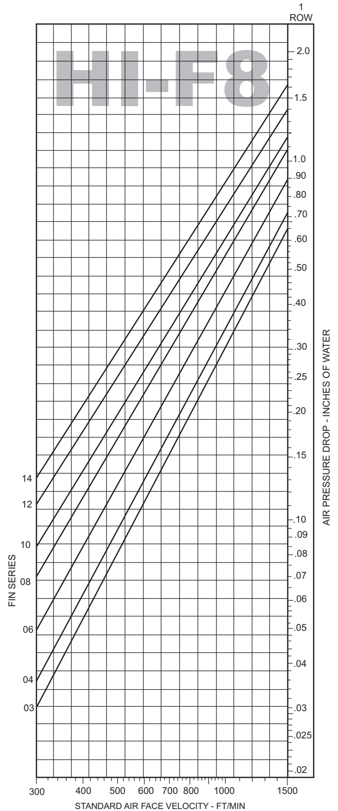
Figure 22: Coil Air Pressure Drop—E-F5 Fin Type
