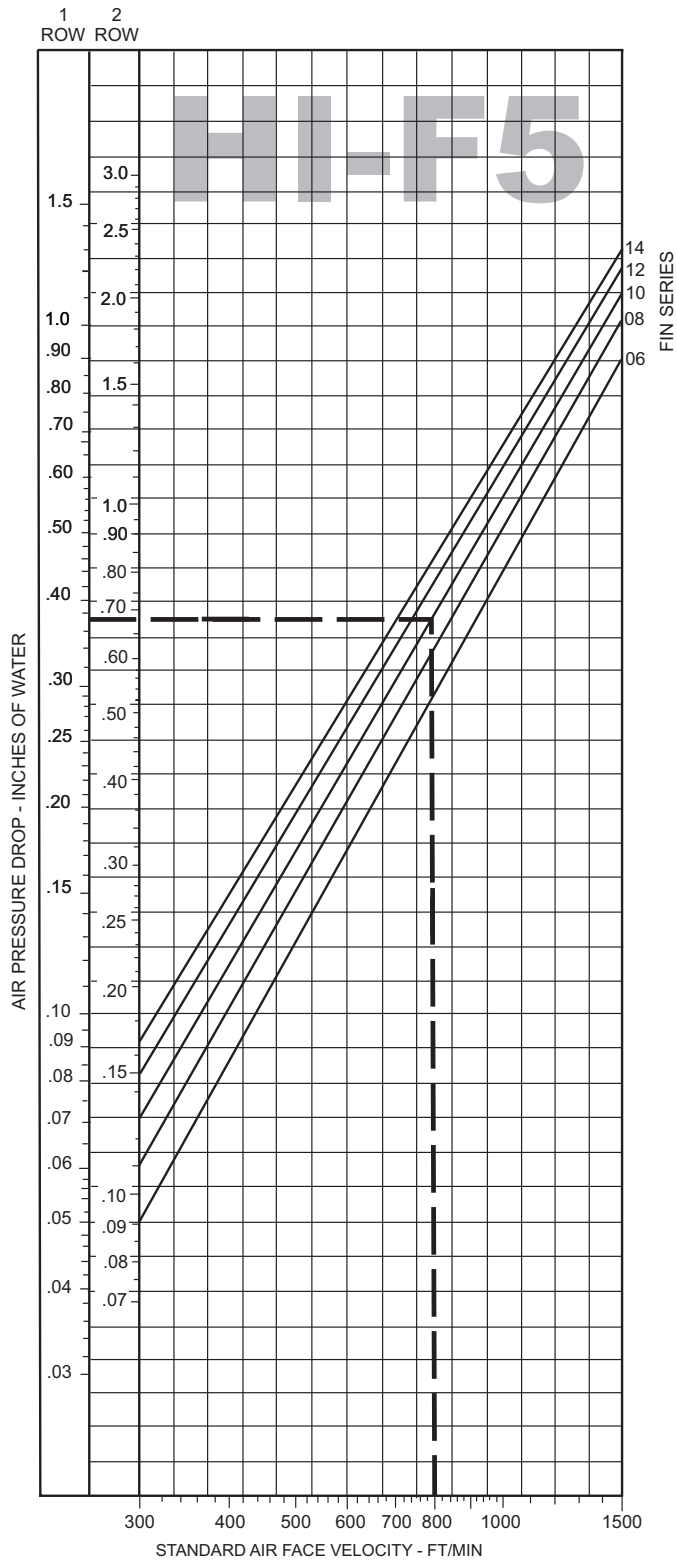
Figure 21: Coil Air Pressure Drop—HI-F5 Fin Type
