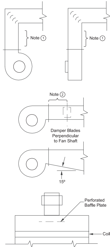
Figure 16: Discharge Duct Layout
