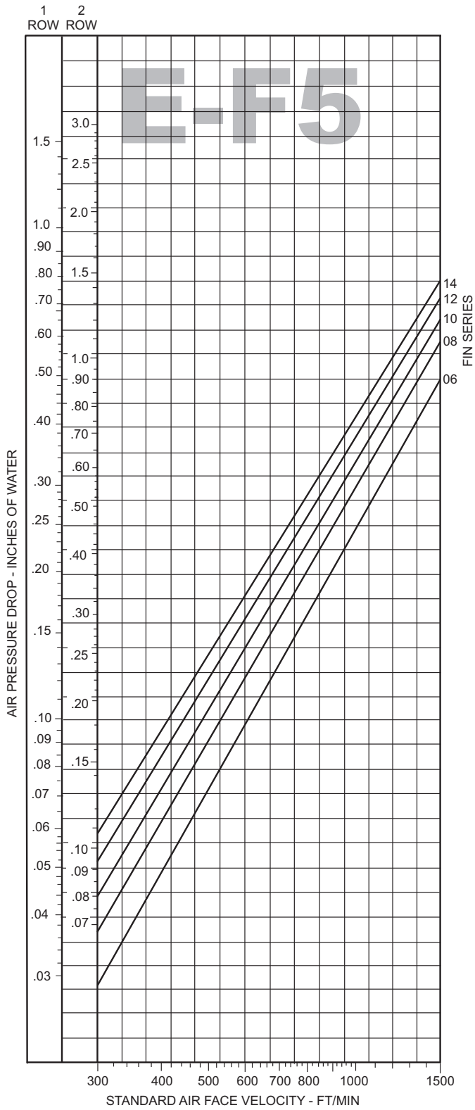
Figure 23: 1" Steam Coil Air Pressure Drop
