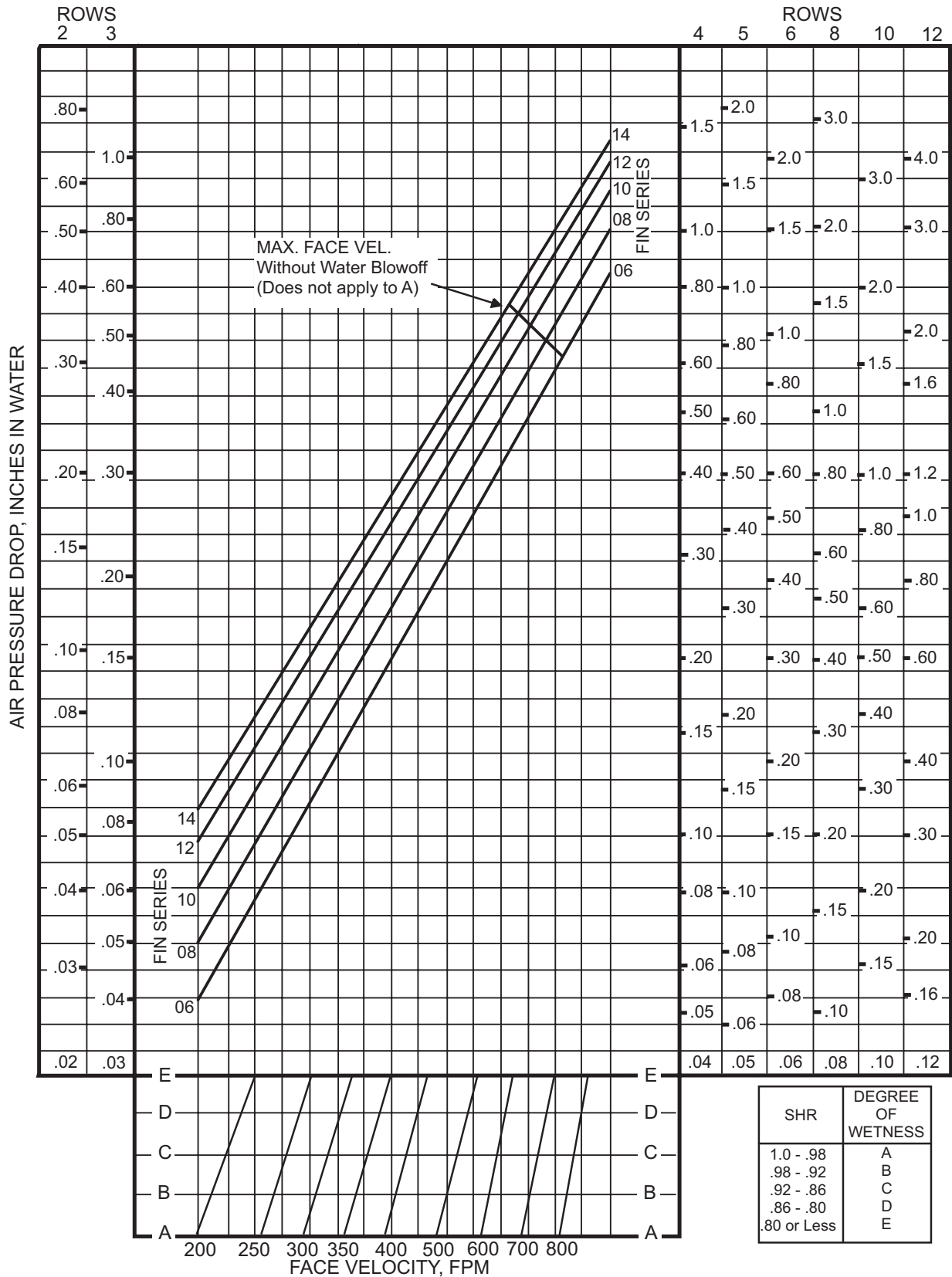
Figure 20: Coil Air Pressure Drop—E-F5 Fin Type (2 Through 12 Rows)
