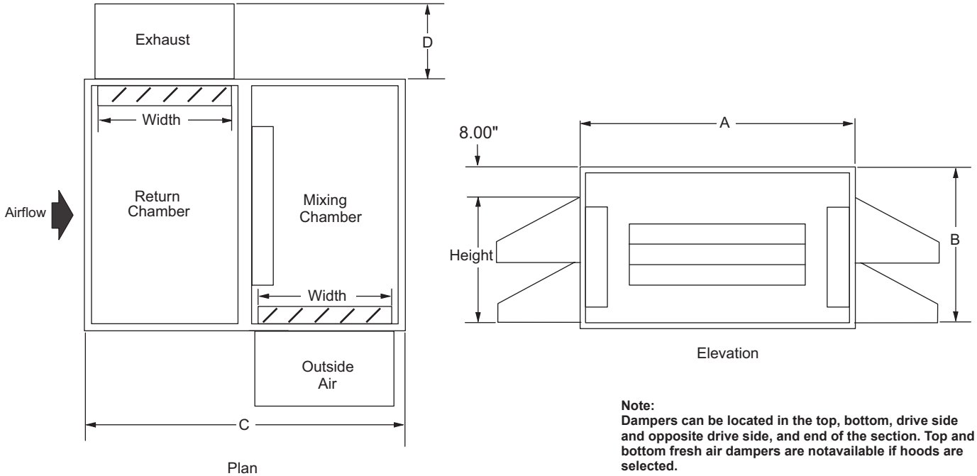
Figure 43: Dimensional Data—Economizer Section, Side Dampers/Hoods
