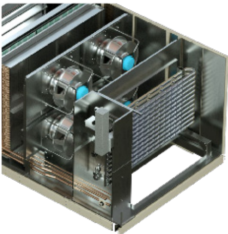
Figure 15: Gas Furnace
