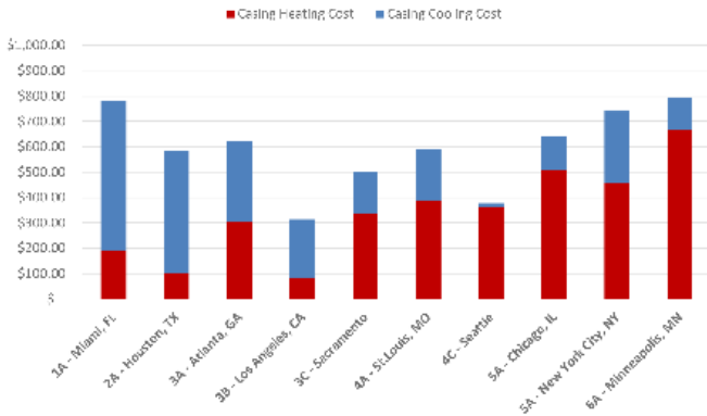
Figure 6: Average Annual Operating Costs of Thermal Losses and Leakage
