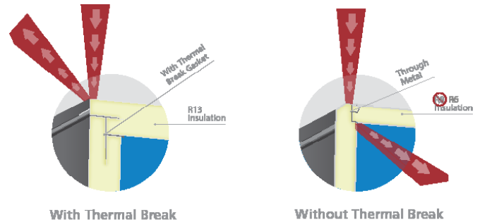
Figure 4: Thermal Break
