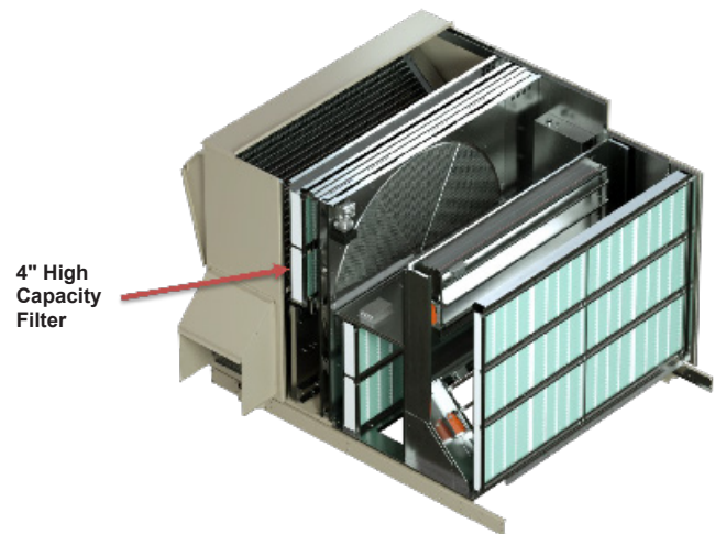
Figure 14: Energy Recovery
