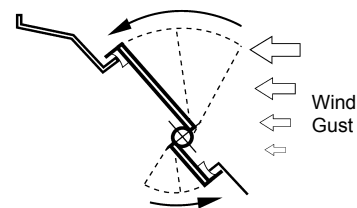
Figure 16: Room Air Damper Auto-Closed by Wind Gusts
