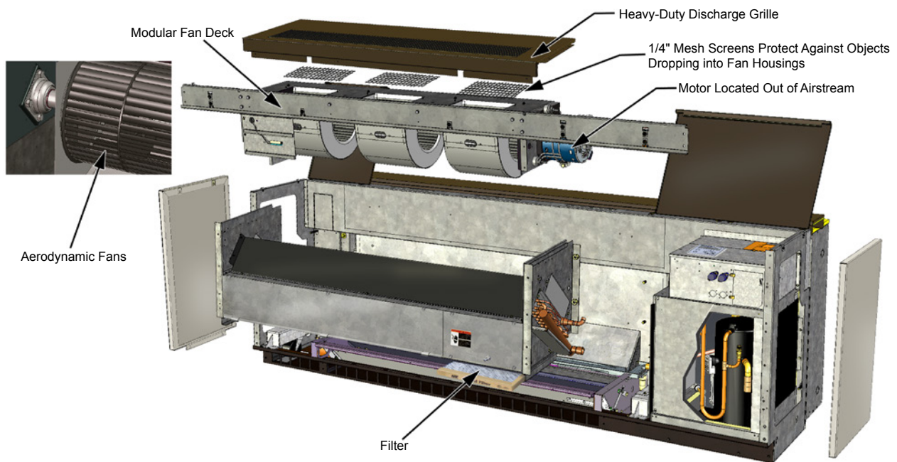
Figure 9: Modular Design
