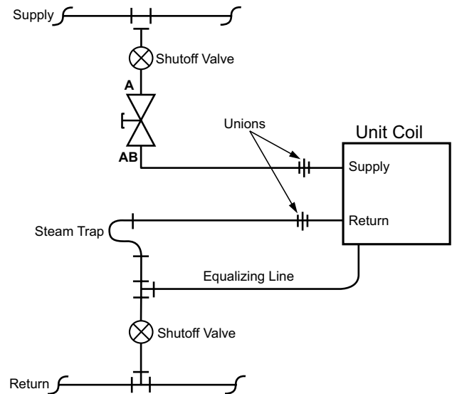
Figure 88: 2-Way Steam Modulating Valve Piping
