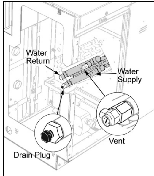
Figure 70: Manual Air Vent & Drain Plug
