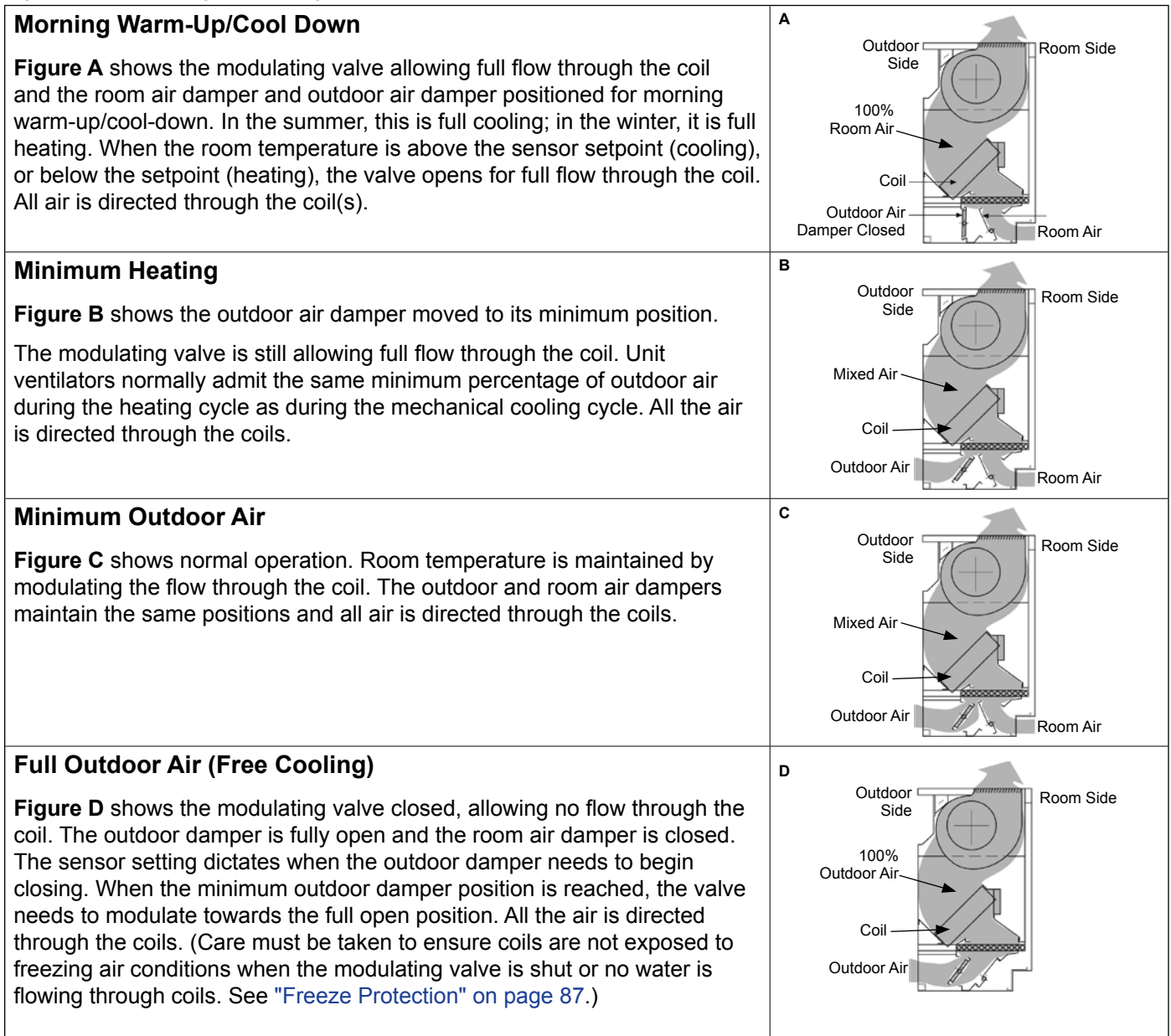
Figure 69: Modulating Valve Temperature Control
