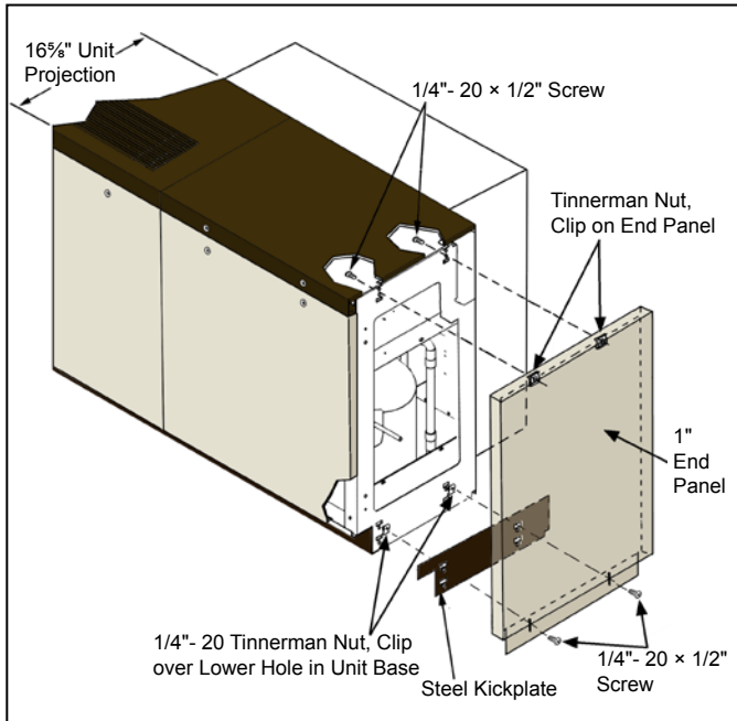
Figure 19: 1" End Panel
