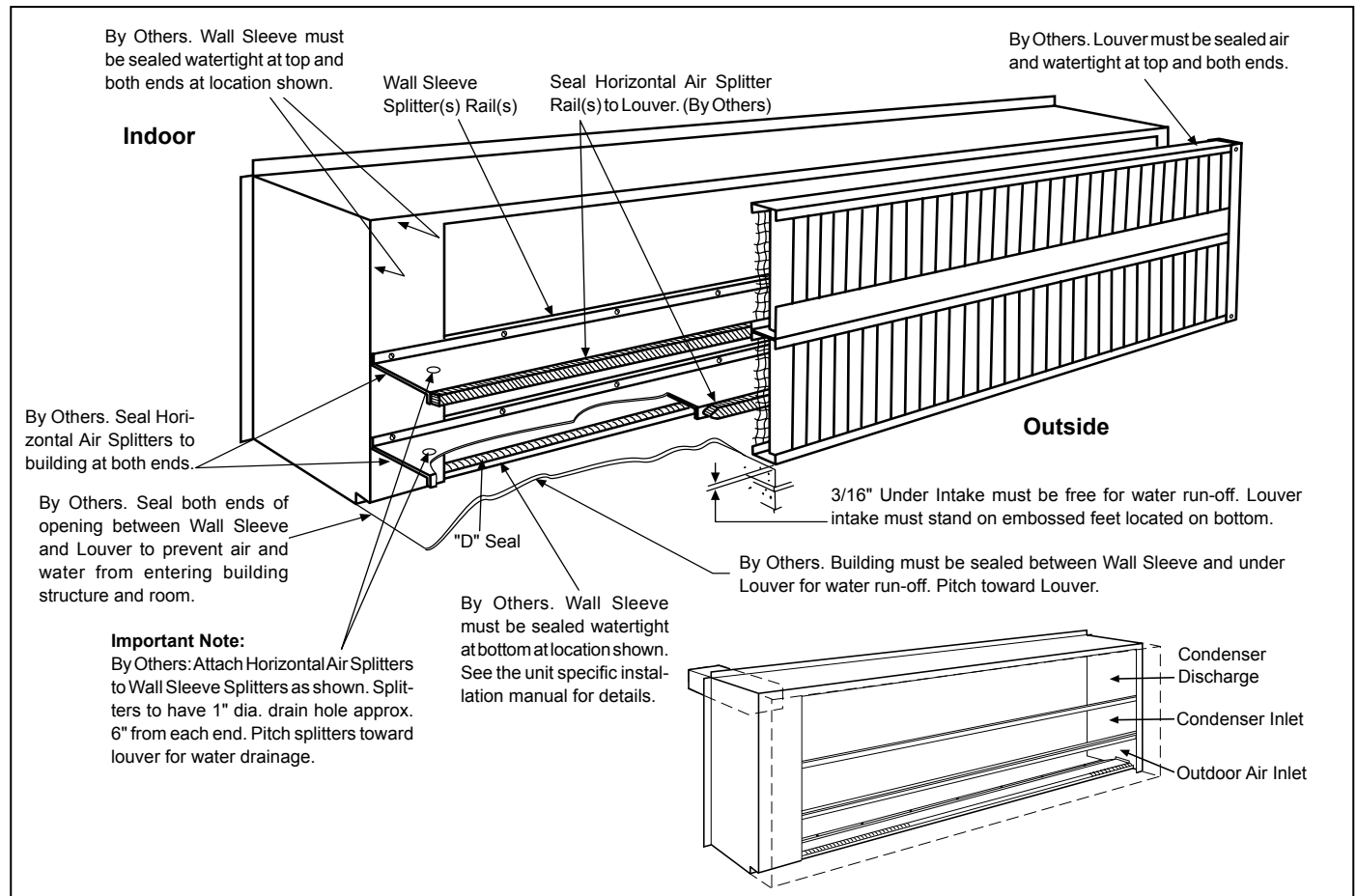
Figure 78: Recessed Wall Sleeve with Horizontal Air Splitters
