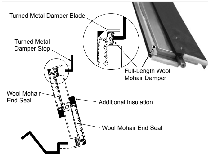
Figure 16: Outdoor Damper Seals Out Cold Weather
