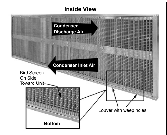
Figure 24: Vertical Blade Louver Inside View, without Flange
