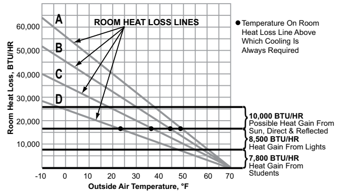
Figure 67: Heat Gain Vs. Heat Loss In Occupied Classrooms
