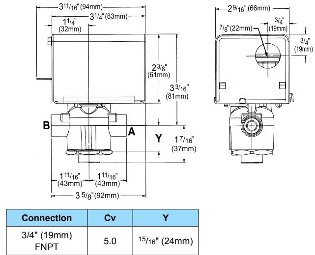
Figure 46: 3-Way EOC Valve Dimensions
