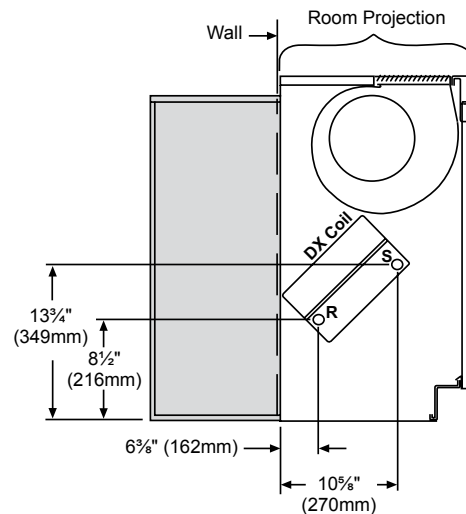
Figure 34: Hot Water Coil Connections – 16 5/8" Type
