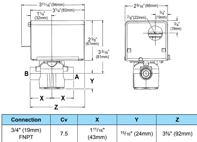
Figure 45: 2-Way EOC Valve Dimensions
