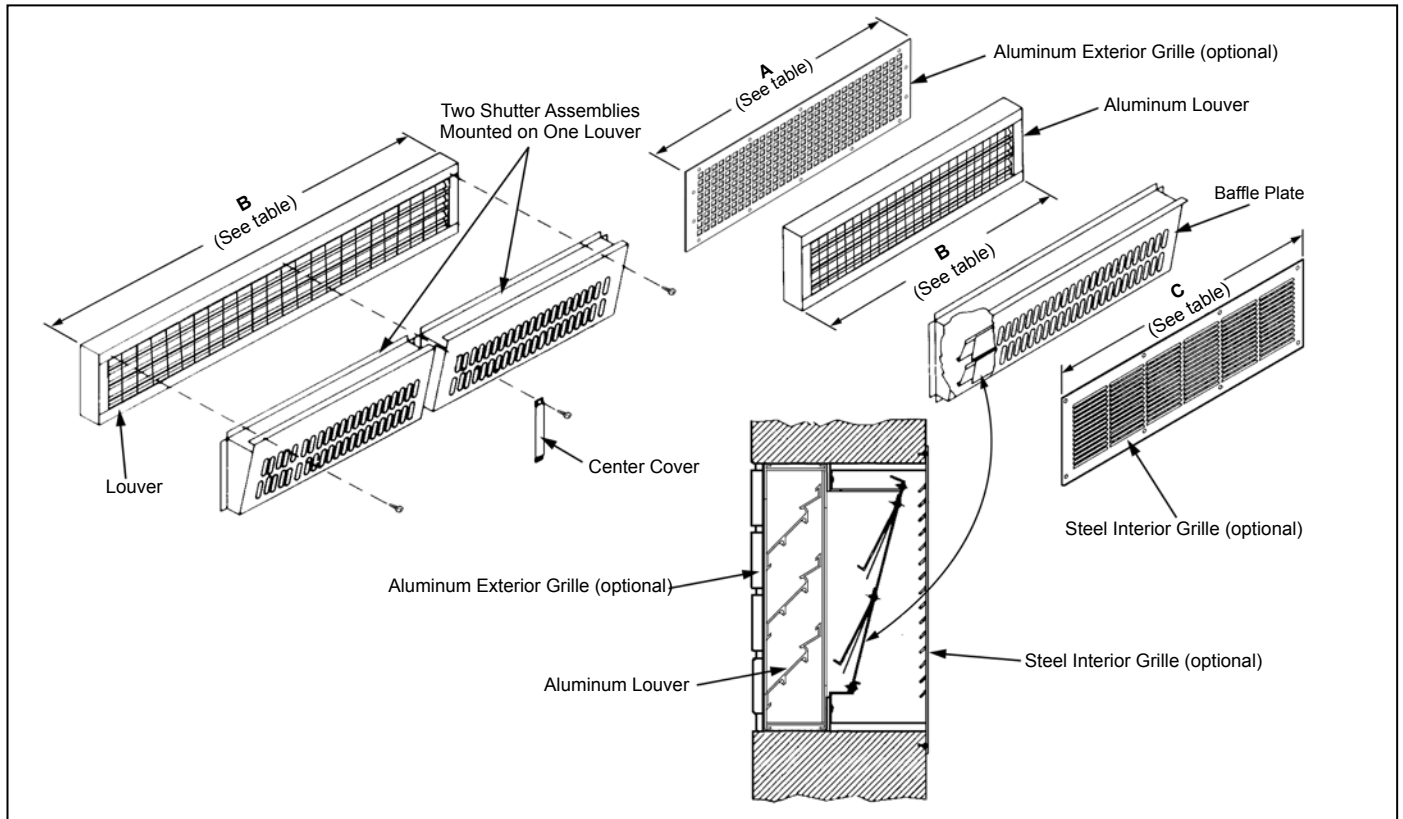
Figure 30: VentiMatic Shutter Assembly with Optional Grille
