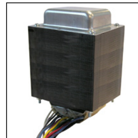
Figure 15: Multi-Tap Auto-Transformer
