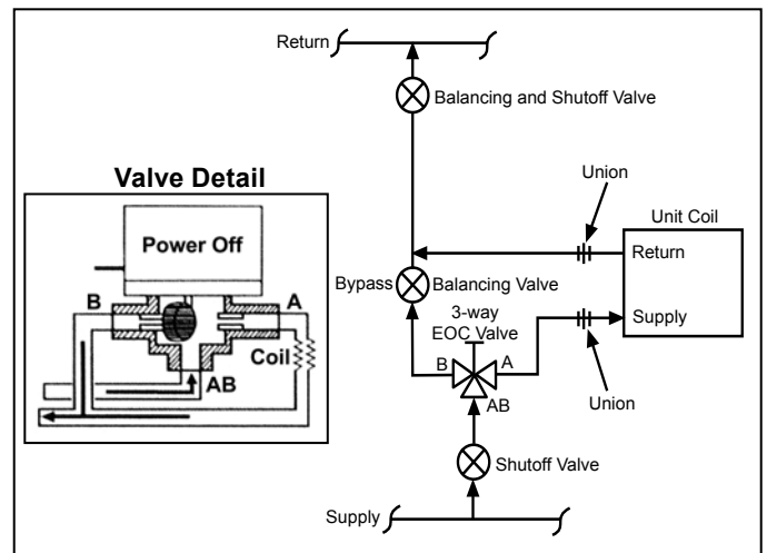
Figure 84: 3-Way Hot Water EOC Valve Piping
