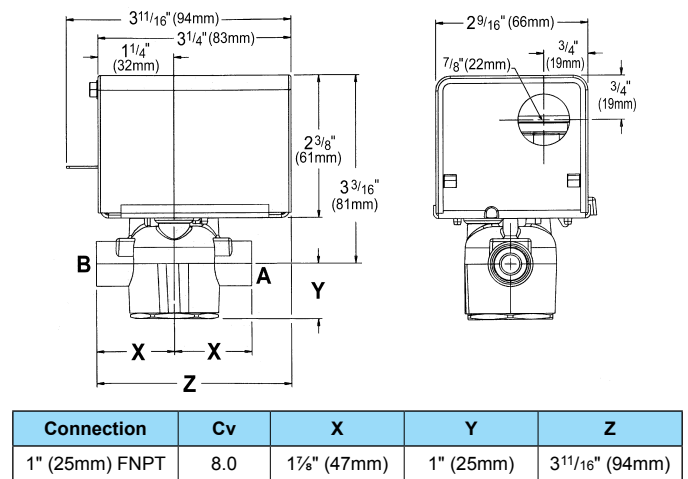
Figure 47: 2-Way EOC Steam Valve Dimensions
