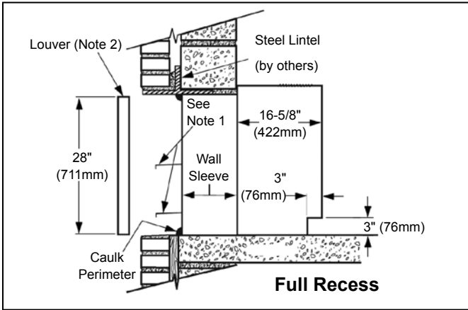
Figure 73: Wall Penetrations Detail
