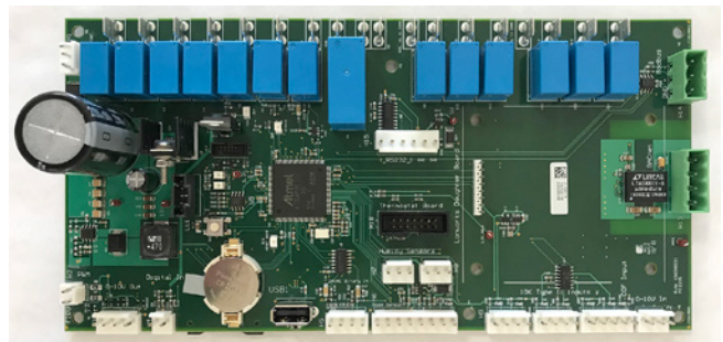
Figure 59: MicroTech Control Board
