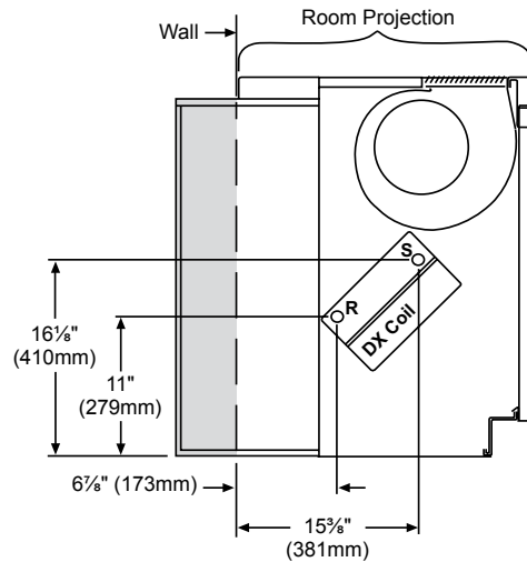
Figure 37: Hot Water Coil Connections – 19 5/8" Type
