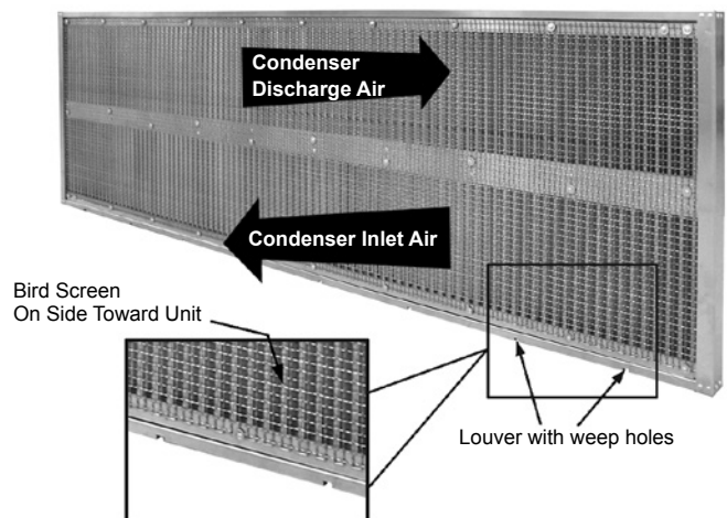
Figure 28: Vertical Blade Louver, without Flange Inside View
