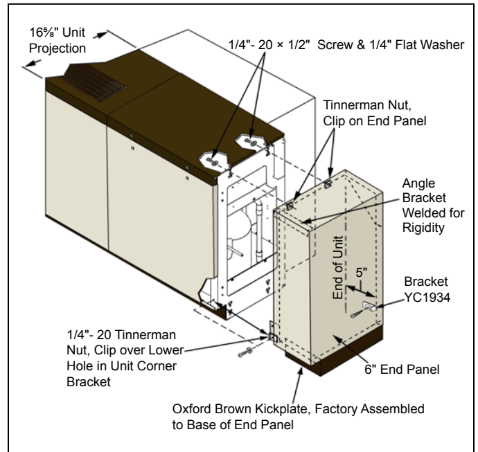
Figure 20: 6" End Panel
