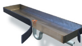
Vertical unit drain pan
