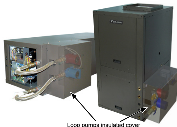
Loop pumps insulated cover
