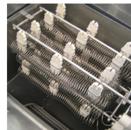
Vertical unit internal factory-installed electric heater
