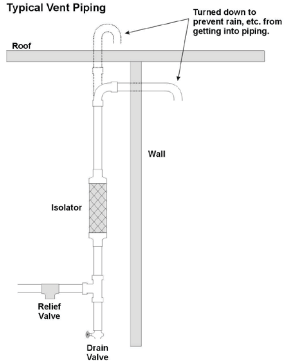
Figure 16: Typical Vent Piping
