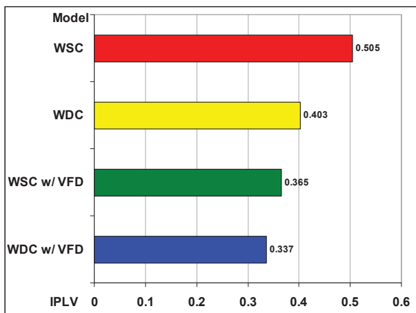
Figure 9: IPLV Comparison by Model
