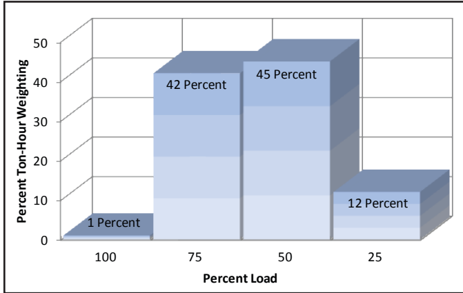
Figure 15: IPLV Defined by AHRI Standard 550/590
