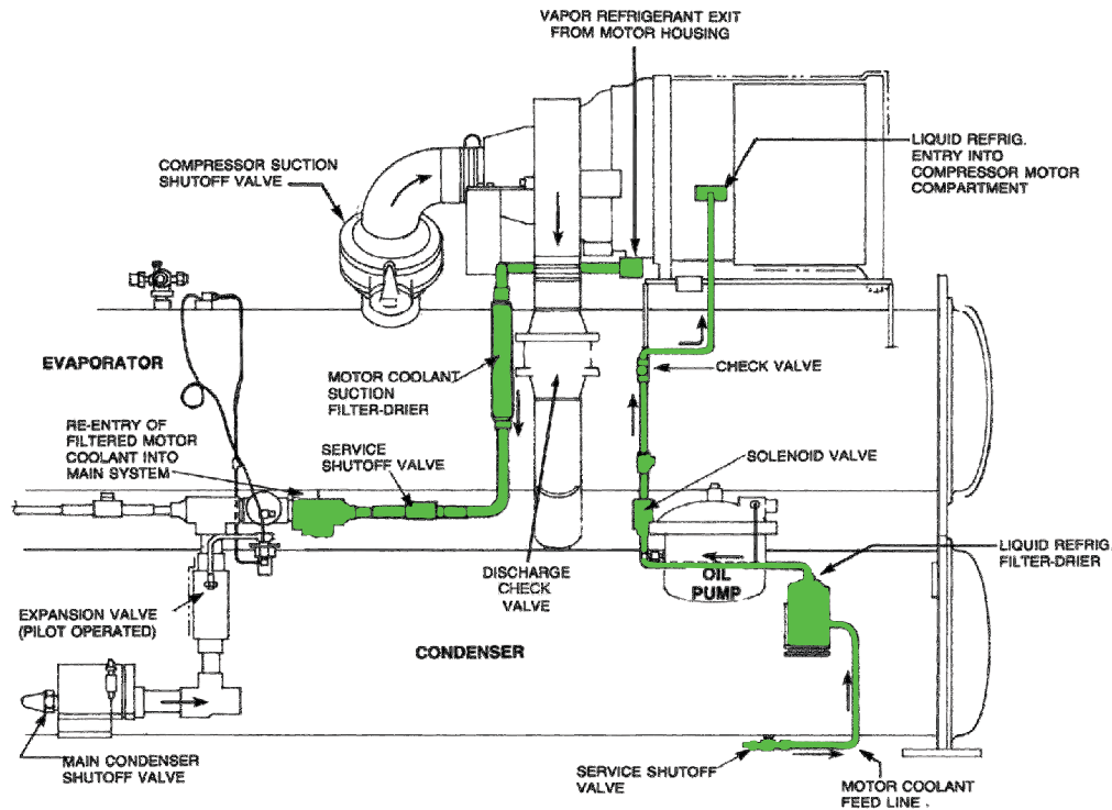
Figure 6: WDC Motor Cooling
