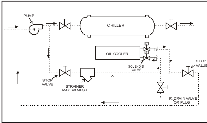
Figure 14: WDC/WCC Oil Cooler Piping With City Water
