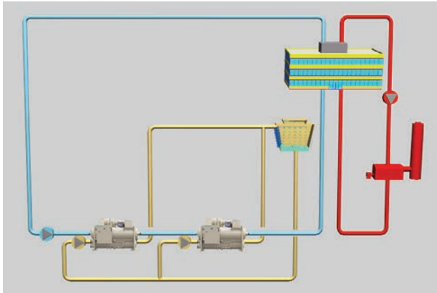
Figure 11: Series Parallel Flow
