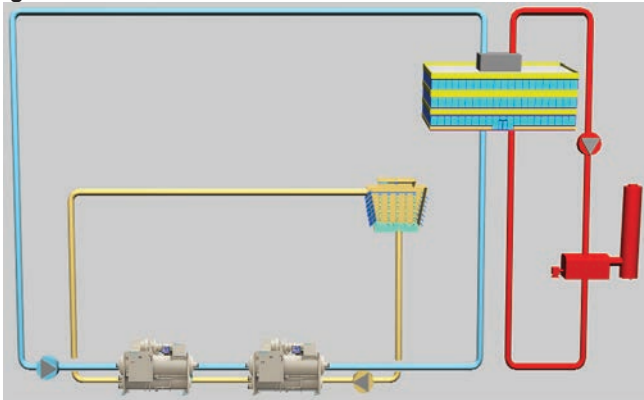
Figure 12: Series Counterflow Flow
